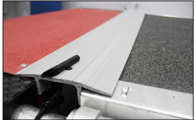
Spacefiller called the new transition piece for scaffolding from Nordic Platform. Photo: Kim Ebbesen.
