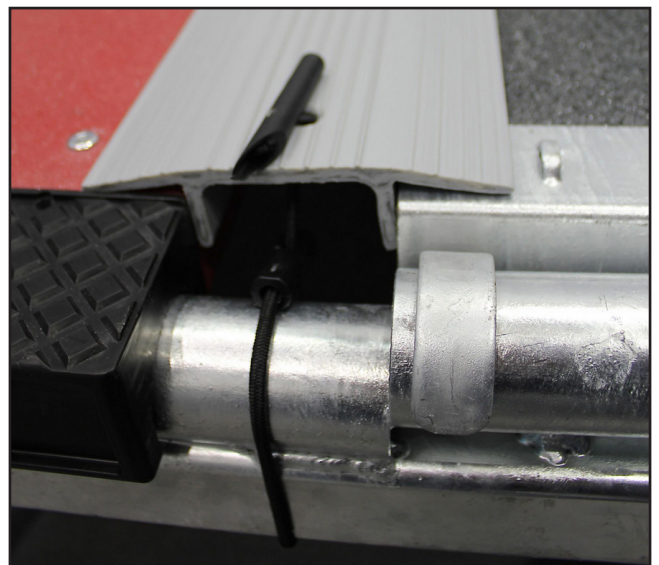
The rail comes in lengths of six meters and can be cut in length with a handsaw. They are fixed easily with straps. Photo: Kim Ebbesen.
